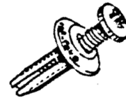
85-5991 Replaces: 90684-SA5-003, 10998-30880, 874-298-1190 RIVET- SCREW TYPE HEADLAMP HOUSING TO GRILLE , Plastic Hole: M5, Washer Head: 15MM Grip Range: 2.0MM - 6.0MM Honda Accord '84/ Nissan: Isuzu, Various Applications UNIT PACKAGE 25
