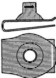
J06216 #10-24 SCREW P.R.: .140-.160, Black Finish UNIT PACKAGE 50
