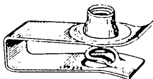
77-4679 Replaces: 1494252 U-NUT-GRILLES Installation in Fiberglass Sections 1/4-20, P.R.: .210 - .330 Ford Trucks & Vans UNIT PACKAGE 50
