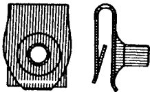
95-7378 Replaces: 45262-S2 NUT-HEADLIGHT RETAINING Formerly 77-4727 #8-32, P.R.: .025 - .150, Throat: .390 Black Finish Ford & General Purpose UNIT PACKAGE 25
