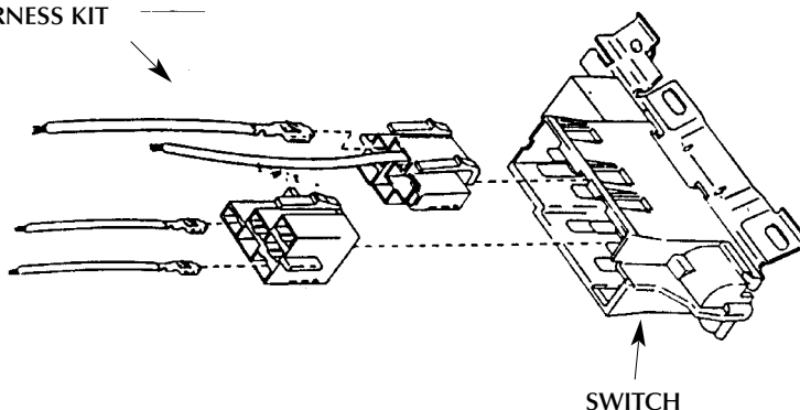
SWITCH
