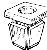
80-5236 Replaces: 26023-H1000 NUT-HEADLAMP ADJUSTING Hole: M8sq., Screw: M4.8 Nissan UNIT PACKAGE 25
