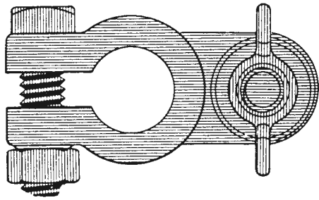
J04423 UNIVERSAL MARINE TYPE BATTERY TERMINAL Fits positive and negative posts. Stud: 3/8" UNIT PACKAGE 10
