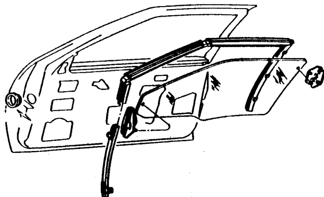
TYPICAL INSTALLATION
