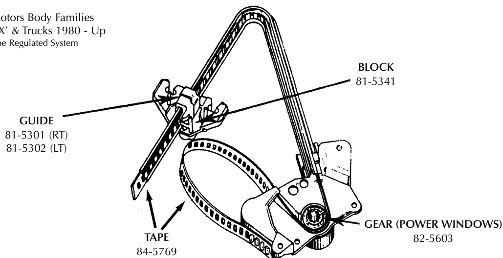
(ILLUSTRATION POWER WINDOW REGULATOR)
