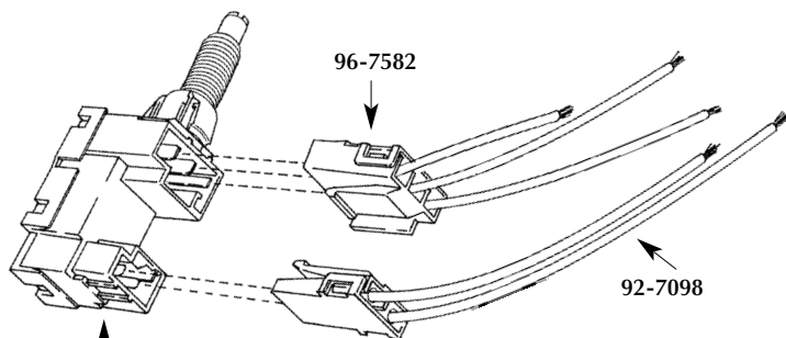
SWITCH
