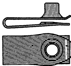
J02463 1/4"-20 BOLT P.R.: .025-.150, Black Finish UNIT PACKAGE 50
